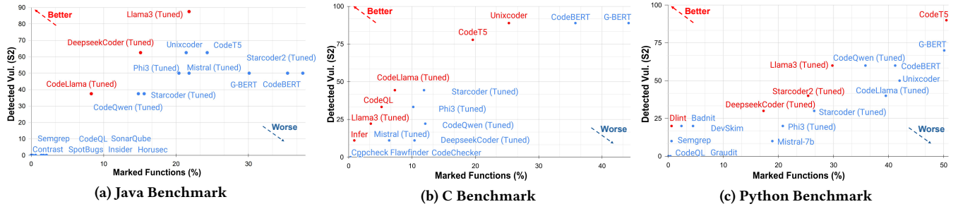
Figure 3: The Relationship between the Vulnerability Detection Ratios (Scenario 2) and the Marked Function Ratios
